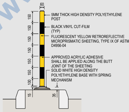
SPRING LOADED POST FOR NARROW DIVIDER (<700mm WIDE)
