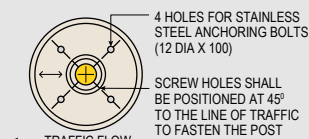
BASE - (PLAN VIEW)
